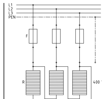
picture 14: connection diagram without thermostat – 400 V \triangle
