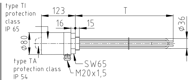
picture 5: type EH (TA/TI) – G 1 1/2" with temperature control for external or internal setting, respectively
