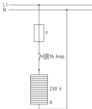
picture 7: connection diagram with thermostat – 230 V
