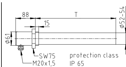
picture 2: type EHP – G 2" without temperature control
