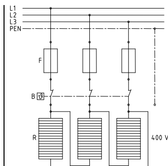
picture 12: connection diagram with thermostat – 400 V \triangle
