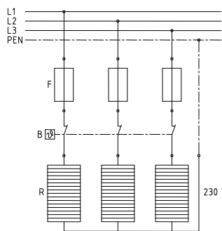
picture 11: connection diagram with thermostat – 230 V \star
