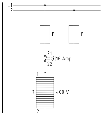
picture 8: connection diagram with thermostat – 400 V
