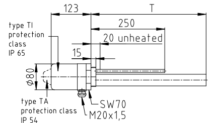
picture 3: type EHP (TA/TI) – G 2" with temperature control
