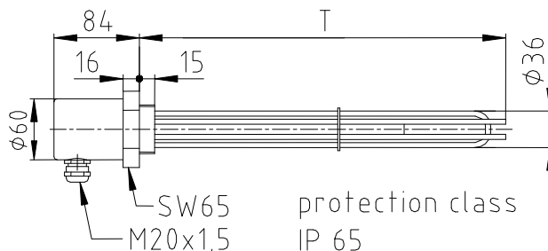
picture 4: type EH – G 1 1/2" without temperature control
