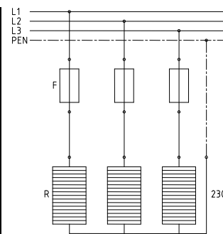
picture 13: connection diagram without thermostat – 230 V \star
