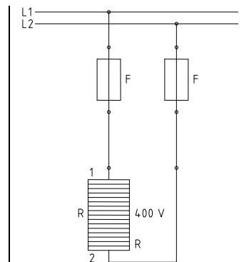
picture 10: connection diagram without thermostat – 400 V
