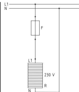
picture 9: connection diagram without thermostat – 230 V
