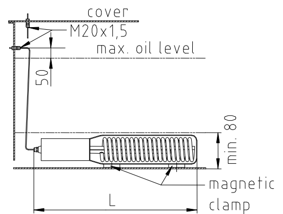
picture 6: installation diagram – TEHM
