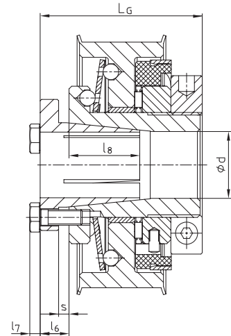
Hub design 4.5
